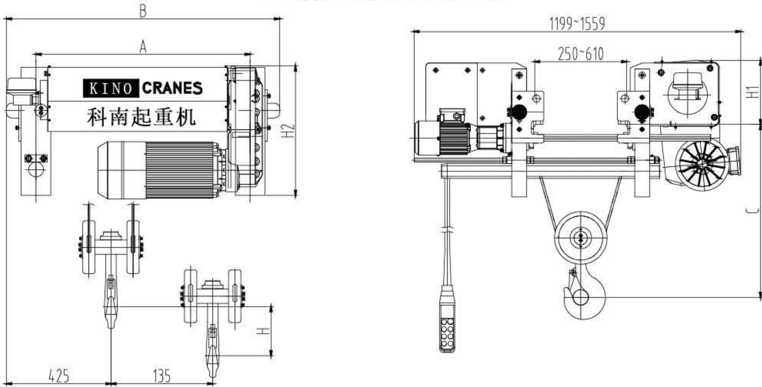
XKD Type European Hoist Sketch
